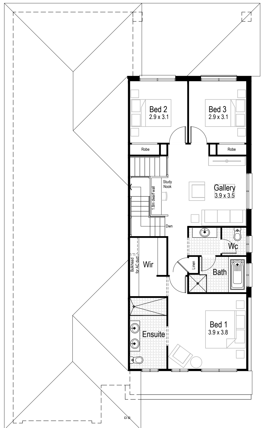
First Floor
